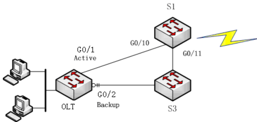
Figure 1: FlexLinkLite-enabled network
