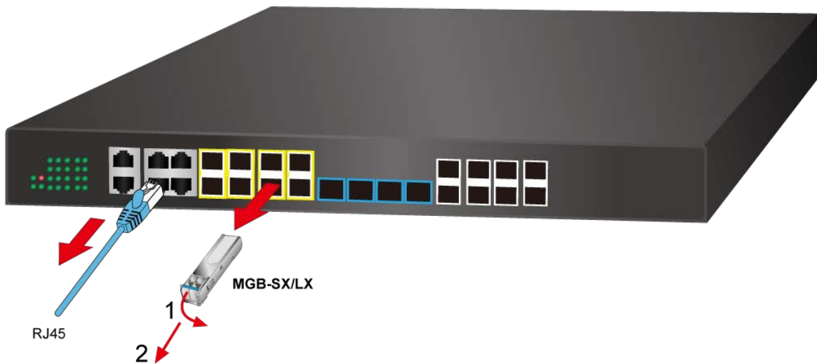
Figure 2-12 Pulling Out the SFP Transceiver
