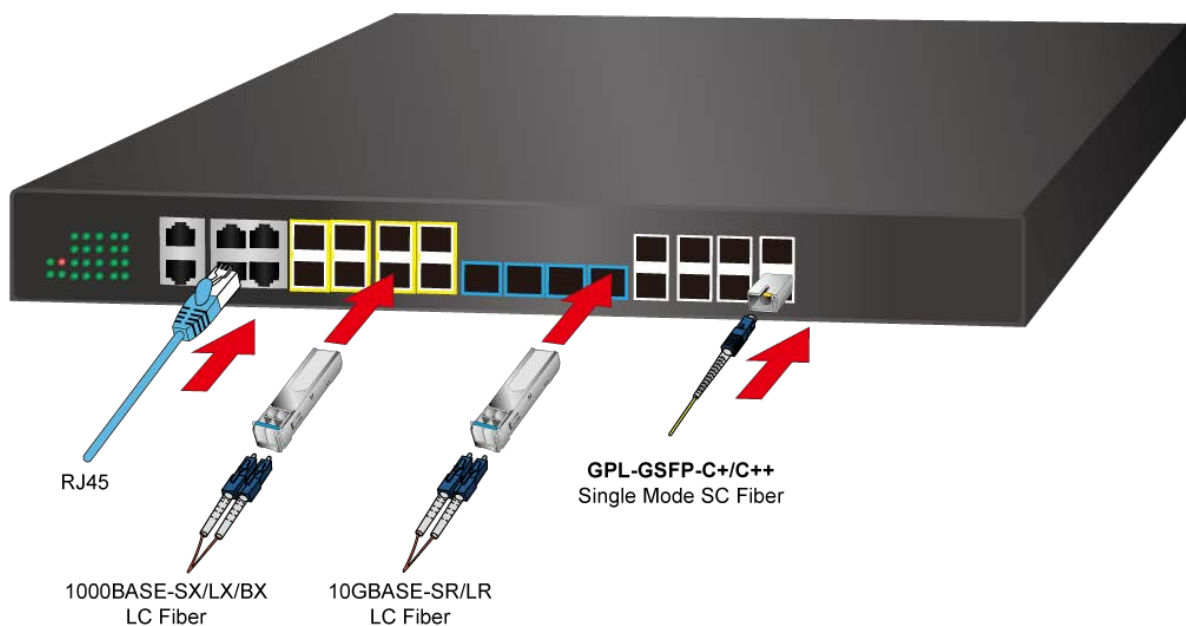
Figure 2-11 Plugging in the SFP Transceiver
