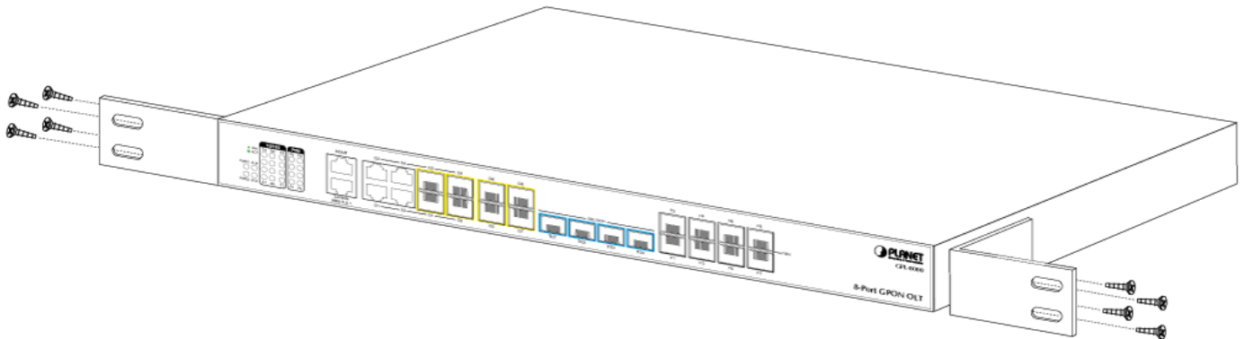
Figure 2-9 Attaching Brackets to the GPON OLT.
